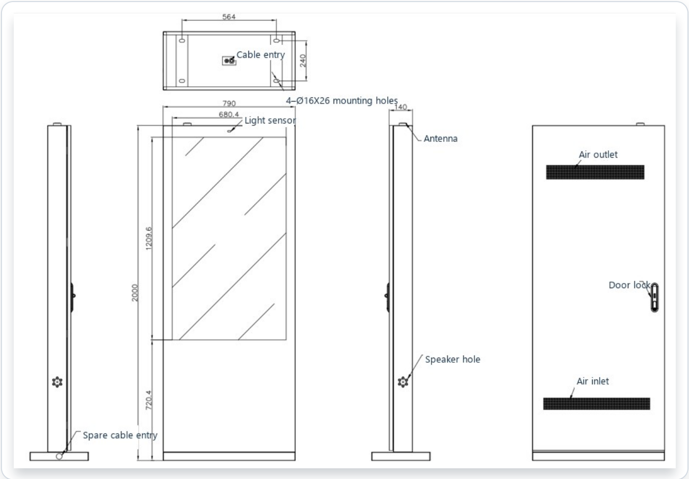
DIMENSIONAL DRAWING · 55" FLOOR-STANDING MODEL, MM
